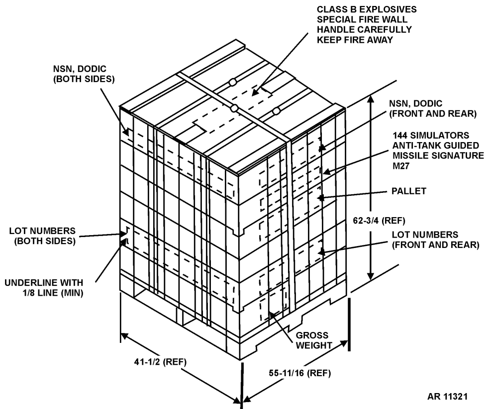
Figure 4-13. Marking for Box, Pallet Type, Wirebound for M27.
