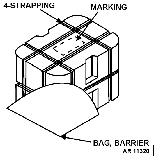
Figure 4-11a. Marking for M27 Foam Support Box.
