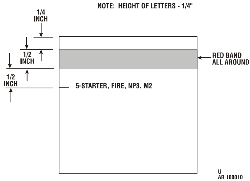
Figure 4-11. Marking for M2 Fire Starter Wooden Packing Box.
